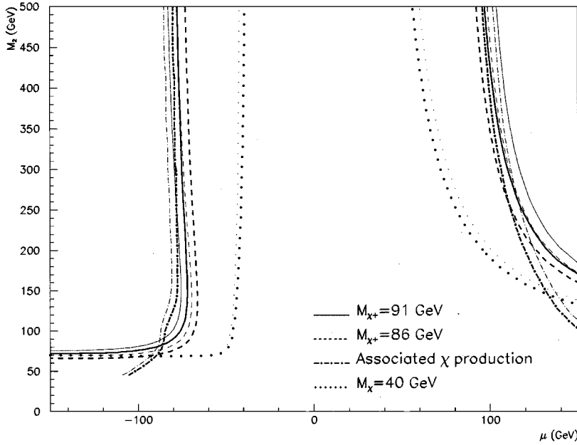
FIG. 1. The effects of one-loop radiative corrections in the \mu, M_2 plane, calculated for \tan \beta = 2 , m_0 = 200 GeV, m_A = 1 TeV, and A_t = 2m_{1/2} . The thick lines are one-loop corrected contours corresponding to fixed values of chargino and neutralino masses, and the thin lines are tree-level contours. The continuous lines are for m_{\chi^\pm} = 91 GeV, the dashed lines for m_{\chi^\pm} = 86 GeV, the dash-dotted lines for the bound on associated neutralino production, and the dotted lines for m_\chi = 40 GeV.
