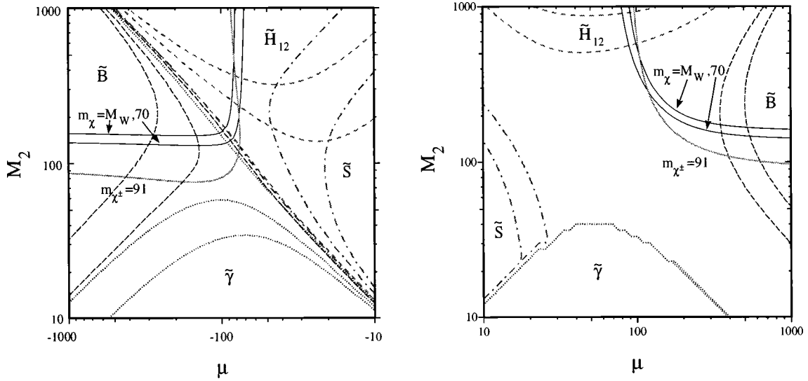
FIG. 4. Contours of neutralino purity: 99, 97, and (for \mu < 0 ) 75 %, and chargino and neutralino masses (solid lines). The long-dashed lines are contours of high bino purity, the dotted lines are contours of high photino purity, the dashed lines are contours of high \tilde{H}_{12} Higgsino purity, and the dash-dotted lines are contours of high \tilde{S}_0 Higgsino purity. The radiative corrections to m_\chi are calculated for \tan \beta = 2 and m_0 = 100 GeV.
