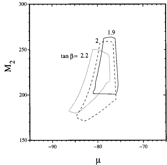
FIG. 6. The regions of the \mu, M_2 plane allowed by the constraints shown in the previous figure are shown for several different values of \tan \beta . There are no consistent choices of Higgsino parameters for \tan \beta < 1.8 or > 2.5 for \mu < 0 , or for any value of \tan \beta for \mu > 0 .
