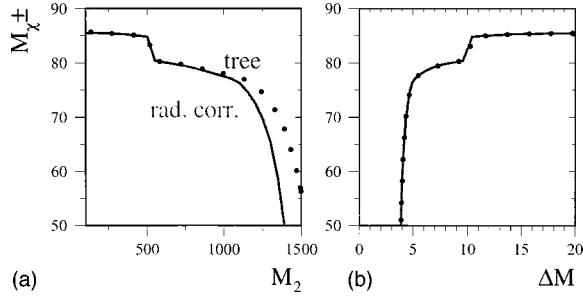
FIG. 2. (a) The experimental limit on m_{\chi^\pm} as a function of M_2 and as a function of \Delta M \equiv m_{\chi^\pm} - m_\chi for fixed m_0 = 200 GeV and \tan \beta = 2 . The value of \mu is determined by the combination m_{\chi^\pm} and M_2 . The drop at large M_2 is due to the loss in experimental efficiency as \chi^\pm decays into \chi involve softer leptons. The dotted line comes from a tree-level analysis, and the solid line is obtained using an ad hoc parametrization of the experimental efficiency, in conjunction with the radiatively corrected mass formulas. Note that the lines separate significantly when M_2 is large. (b) The experimental limit on m_{\chi^\pm} is now plotted as a function of \Delta M \equiv m_{\chi^\pm} - m_\chi . Note that the tree-level and radiatively corrected curves are almost coincident.
