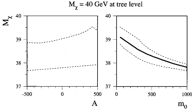
FIG. 3. Plots of the radiative correction to the lower limit on the neutralino mass, in the case that m_{\chi^\pm} = 85 GeV; \tan \beta = 2 and \mu = -140 GeV. The plots are obtained by varying -500 \text{ GeV} \leq A_t \leq 500 \text{ GeV} and 50 \text{ GeV} \leq m_0 \leq 1000 \text{ GeV} . The solid line in the second panel is for the fixed-point value A_t = 2m_{1/2} . We see that the limit on m_\chi is reduced by about 1 GeV if we assume this value of A_t and take m_0 = 80 GeV, corresponding to the tree-level lower limit on m_\chi .
