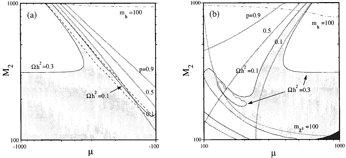
FIG. 7. Larger regions of the \mu, M_2 plane for \tan \beta = 2 and (a) \mu < 0 , (b) \mu > 0 , with the radiatively corrected contours for m_{\chi^\pm} = 100 GeV and m_h = 100 GeV, three choices of the Higgsino purity, and the \Omega_\chi h^2 = 0.1, 0.3 contours for m_0 = 100 GeV and [in (a)] 1000 GeV (dashed lines). We see that the allowed regions for gaugino dark matter are very much larger than those for Higgsino dark matter shown in Fig. 5. The small dark shaded region in (b) yields a top squark with a negative mass squared.
