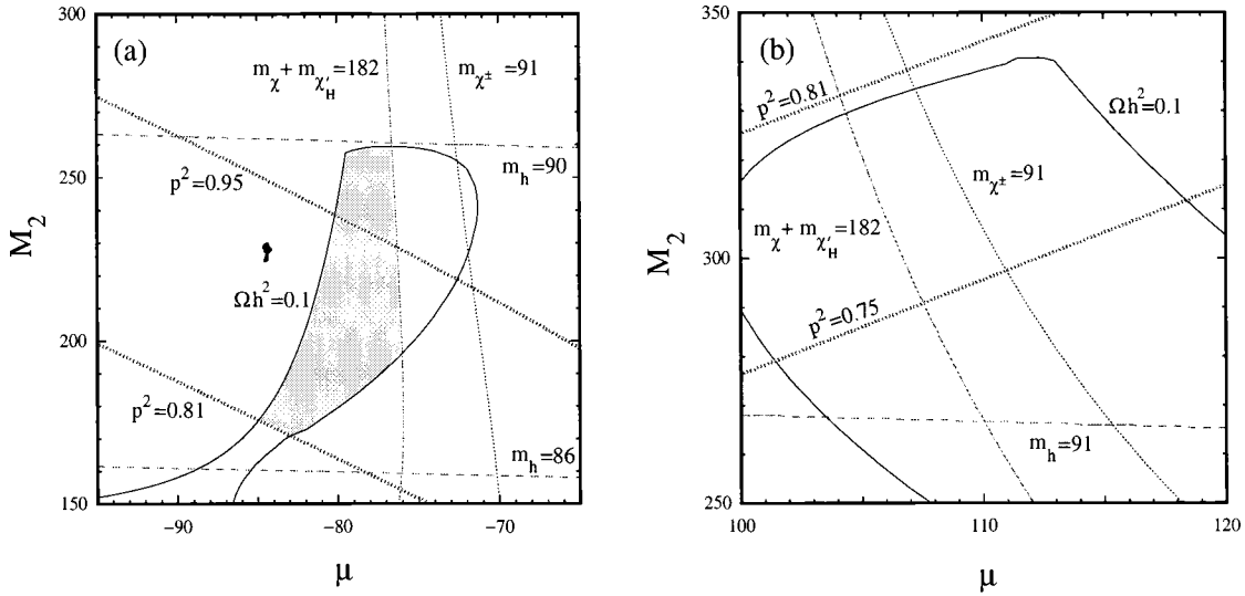
FIG. 5. Survey of experimental and cosmological constraints in the \mu, M_2 plane, focusing on Higgsino dark matter for \tan \beta = 2 and (a) \mu < 0 and (b) \mu > 0 . We plot the radiatively corrected contours for m_{\chi^\pm} = 91 GeV, for m_\chi + m_{\chi'} = 182 GeV, for selected values of m_h and the Higgsino purity p , and for \Omega_\chi h^2 = 0.1 . The shaded regions yield a Higgsino which satisfies the mass and relic density constraints described in the text.
